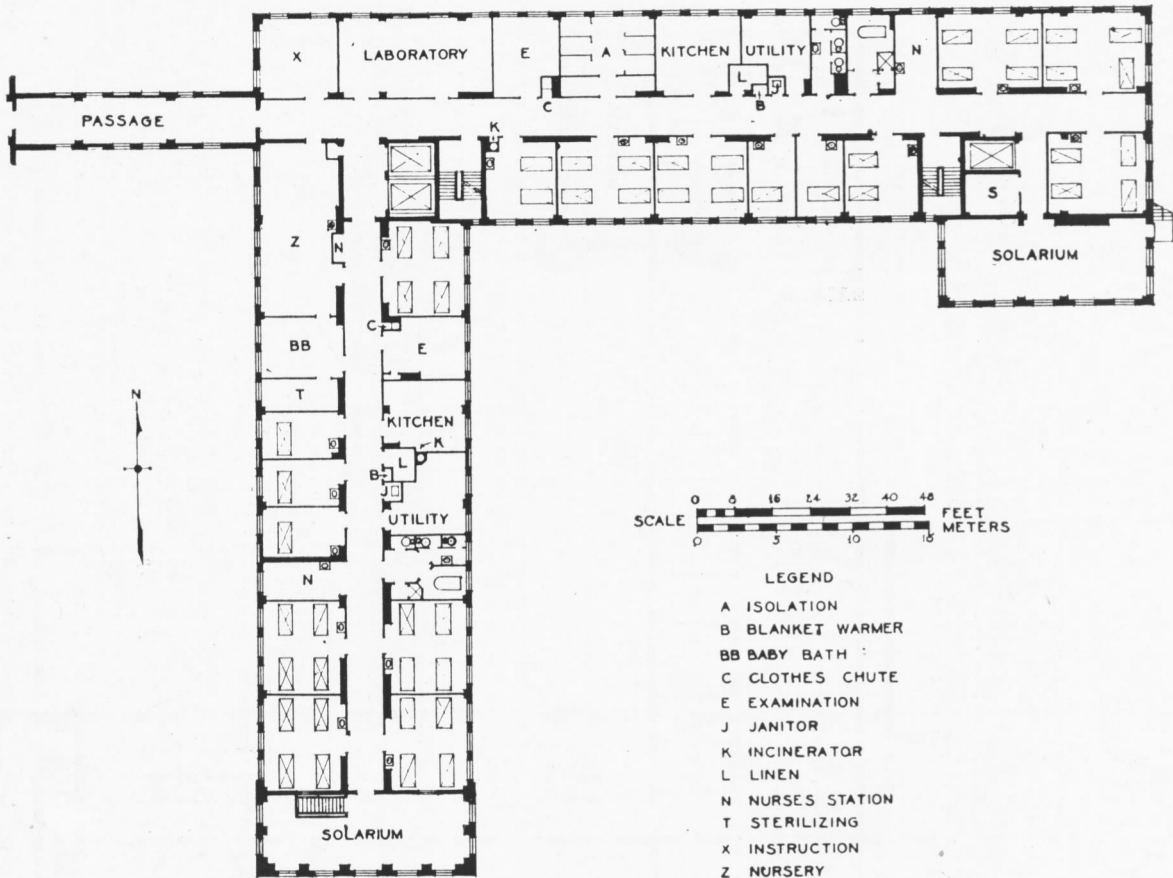
Fig. 161. Plan of Fifth Floor ROCHESTER MUNICIPAL HOSPITAL, Rochester, N. Y. Gordon & Kaelber, Architects
