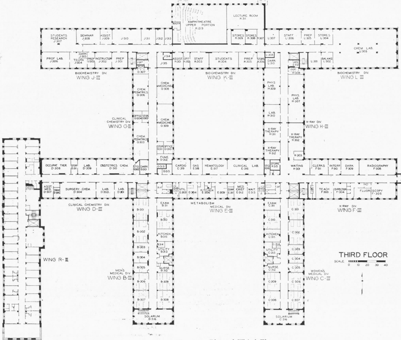
Fig. 153. Plan of Third Floor SCHOOL OF MEDICINE AND DENTISTRY, STRONG MEMORIAL HOSPITAL, ROCHESTER, N. Y. William G. Kaelber and L. A. Waasdorp, Architects
