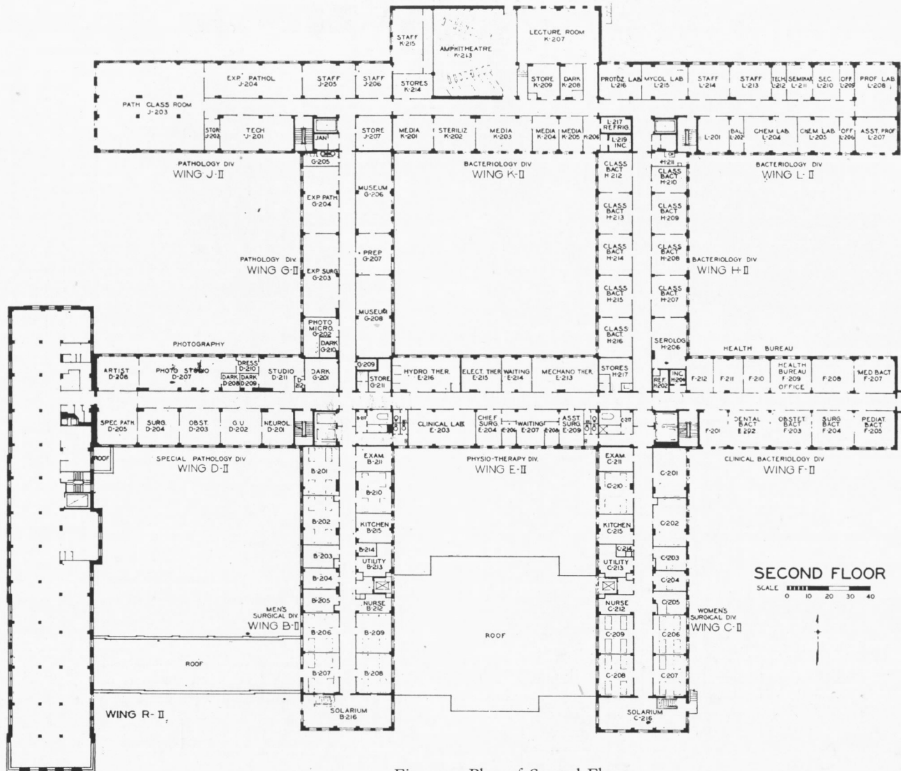
Fig. 152. Plan of Second Floor SCHOOL OF MEDICINE AND DENTISTRY, STRONG MEMORIAL HOSPITAL, ROCHESTER, N. Y. William G. Kaelber and L. A. Waasdorp, Architects
